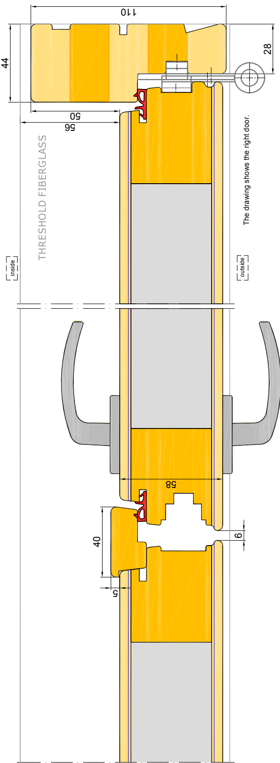
DOOR OUTWARD OPENABLE
